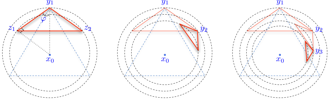
Figure 6: Pyramids constructed by Algorithm 2. First diagram is the initial pyramid constructed by the algorithm at round i of epoch \tau with apex y_1 , base vertices z_1, \dots, z_d and angle \varphi at the vertex. The other diagrams show the subsequent pyramids which successively get closer to the center of the ball
