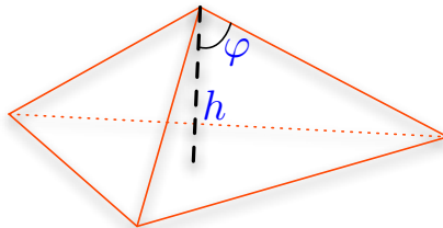
Figure 4: Pyramid in 3-dimensions
