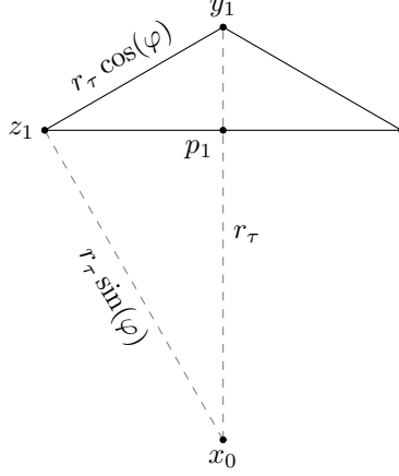
Figure 13: Construction of pyramids.
