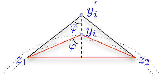
Figure 9: Transformation of the pyramid \Pi in the hat-raising step.
