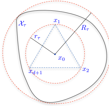
Figure 5: The regular simplex constructed at round i of epoch \tau with radius r_\tau , center x_0 and vertices x_1, \dots, x_{d+1} .
