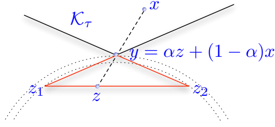
Figure 11: The points of interest in Lemma 5 (see text). Solid lines depict the pyramid \Pi and the \mathcal{K}_\tau .
