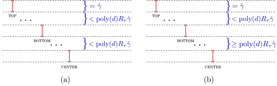
Figure 8: Relative ordering of confidence intervals of TOP, BOTTOM and center CENTER in cases 2(a) and 2(b) of the algorithm resp.
