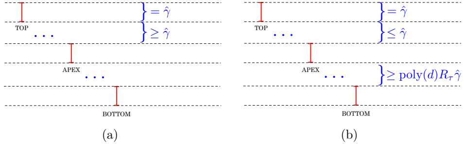
Figure 7: Relative ordering of confidence intervals of TOP, BOTTOM and APEX in cases 1(a) and 1(b) of the algorithm resp.
