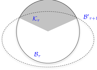
Figure 10: Illustration of the cone-cutting step at epoch \tau . Solid circle is the enclosing ball \mathcal{B}_\tau . Shaded region is the intersection of \mathcal{K}_\tau with \mathcal{B}_\tau . The dotted ellipsoid is the new enclosing ellipsoid \mathcal{B}'_{\tau+1} for the residual domain.
