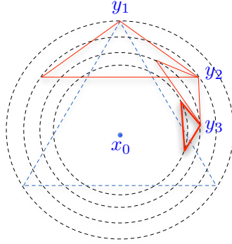
Figure 12: The apexes of the successive pyramids get closer to the center of the simplex x_0 and eventually enter the simplex after at most \mathcal{O}(d^2 \log d) pyramids.
